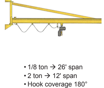
JOWU - Over Braced Wall Mounted Jib With R&M's UKA Profile Beam
