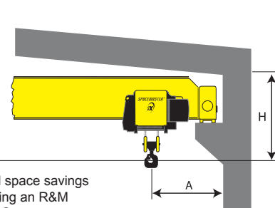
Building with R&M C-track Festoon
