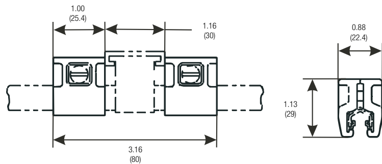
Multi-Conductor Web Bracket
