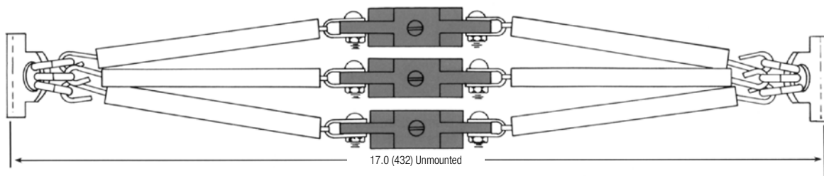
Unmounted Collector Assembly
