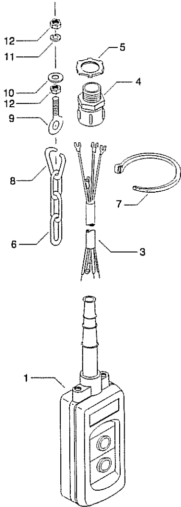
PUSHBUTTON STATION
