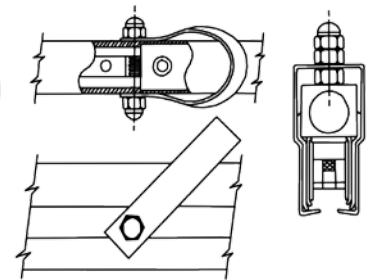
Center Slide Assembly with Cable Strap
